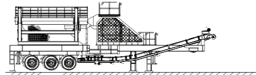
移动破碎站——颚式破碎机 Jaw Crusher Series of Mobile Crusher Plant
