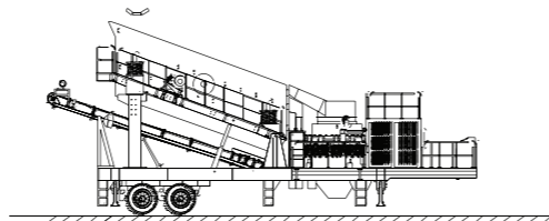
移动破碎站——圆锥式破碎机 Cone Crusher Series of Mobile Crusher Plant
